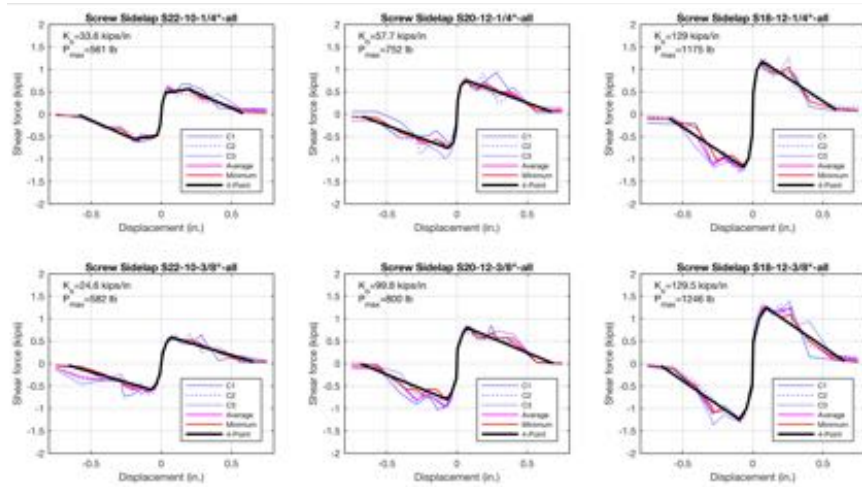
Fig. 12. Average backbone curves of the cyclic tests
