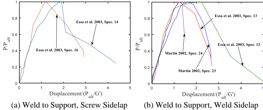
Figure 6. Behavior of Cyclically Loaded Bare Deck Specimens
