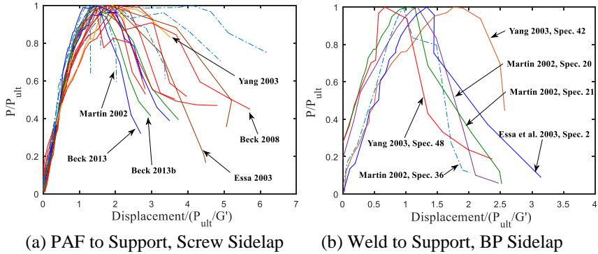
Figure 5. Behavior of Cyclically Loaded Bare Deck Specimens
